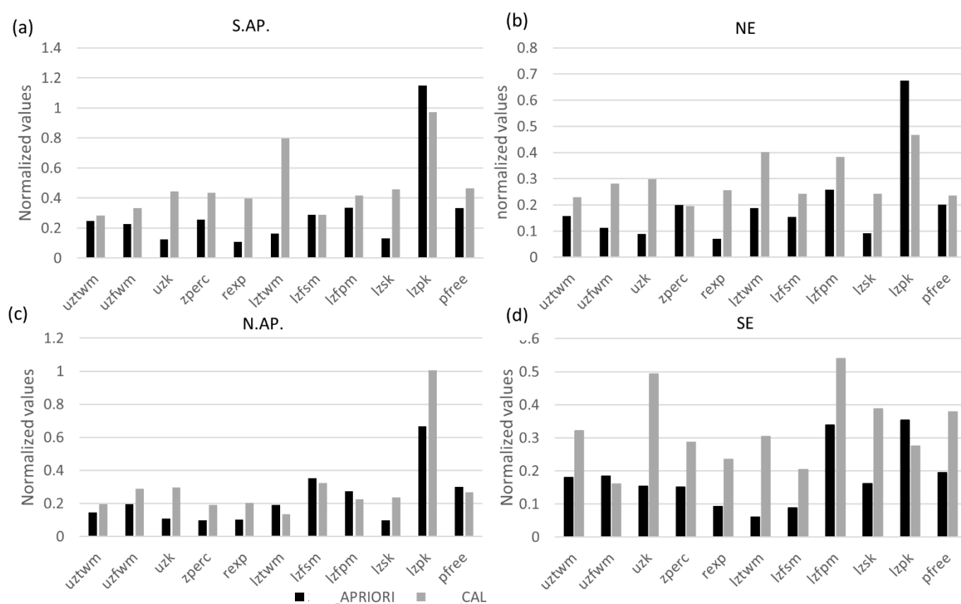
Figure 7. The parameters variability in each region refers to the normalized standard deviations of each parameter by the median of parameters standard deviation in the study region during APRIORI and CAL simulations, respectively. Please refer to Table 2 and Figure 3 for the meaning of each model parameter in Figures (a–d).
